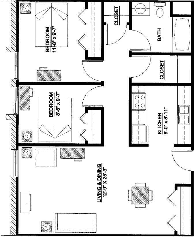
FORT HOWARD APARTMENTS 2 BEDROOM DESIGN SCALE: 1/4" = 1'-0"
